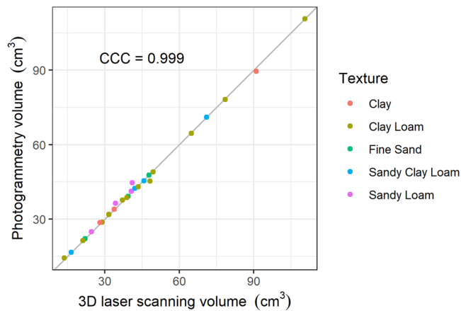
FIGURE 3 Concordance between volume estimates using photogrammetry and laser 3D scanning. The line represents a 1:1 relationship. CCC = concordance coefficient.
