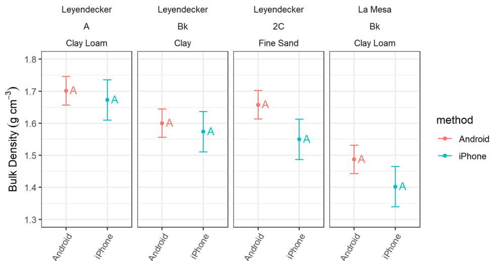
FIGURE 5 Photogrammetry measurements of D_b using two different cameras. Within a panel, means with the same letter are not different at p = 0.05 .
