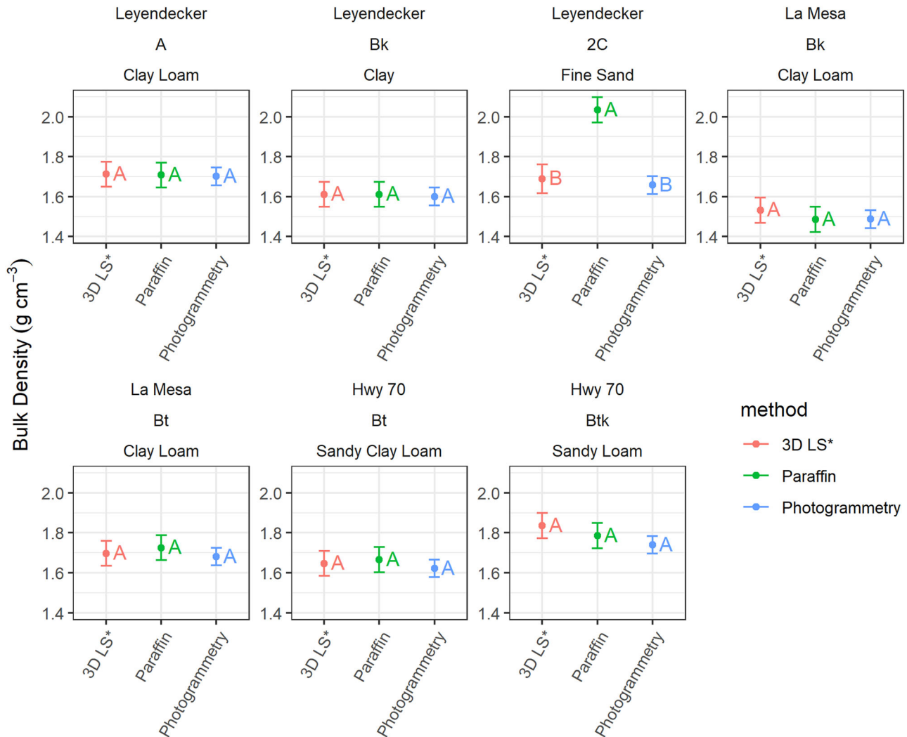
FIGURE 4 Comparison of measured D_b between different methods. Points reflect least squares means and error bars represent \pm 1 standard error from ANOVA analysis. Means with different letters indicate methods with statistically significant ( p < 0.05 ) differences within a panel. Photogrammetry measurements were derived using the android based camera. Photogr. = photogrammetry, 3D LS* = 3D Laser Scanning which was performed on a physically different ped from the same horizon.
